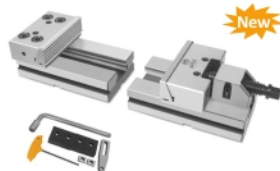
APEX CODE 795 High Precision Two Piece Modular Vice Accuracy 0.02 MM Hardness 57-62 HRC
