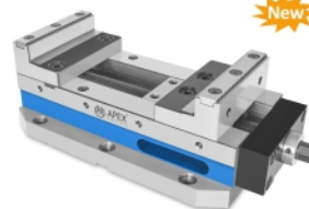
APEX CODE 798 Compact High Grip Vice Accuracy 0.02 MM Hardness 60 ± 2 HRC
