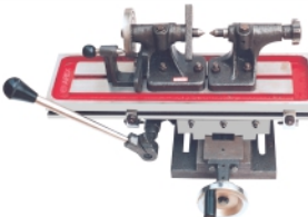
APEX CODE 722D Profiling Milling & Slotting Slide with Indexing Dividing Head and Tail Stock
