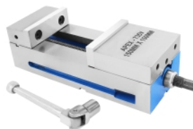
APEX CODE 735 V Precision Tilt Lock Machine Vice
